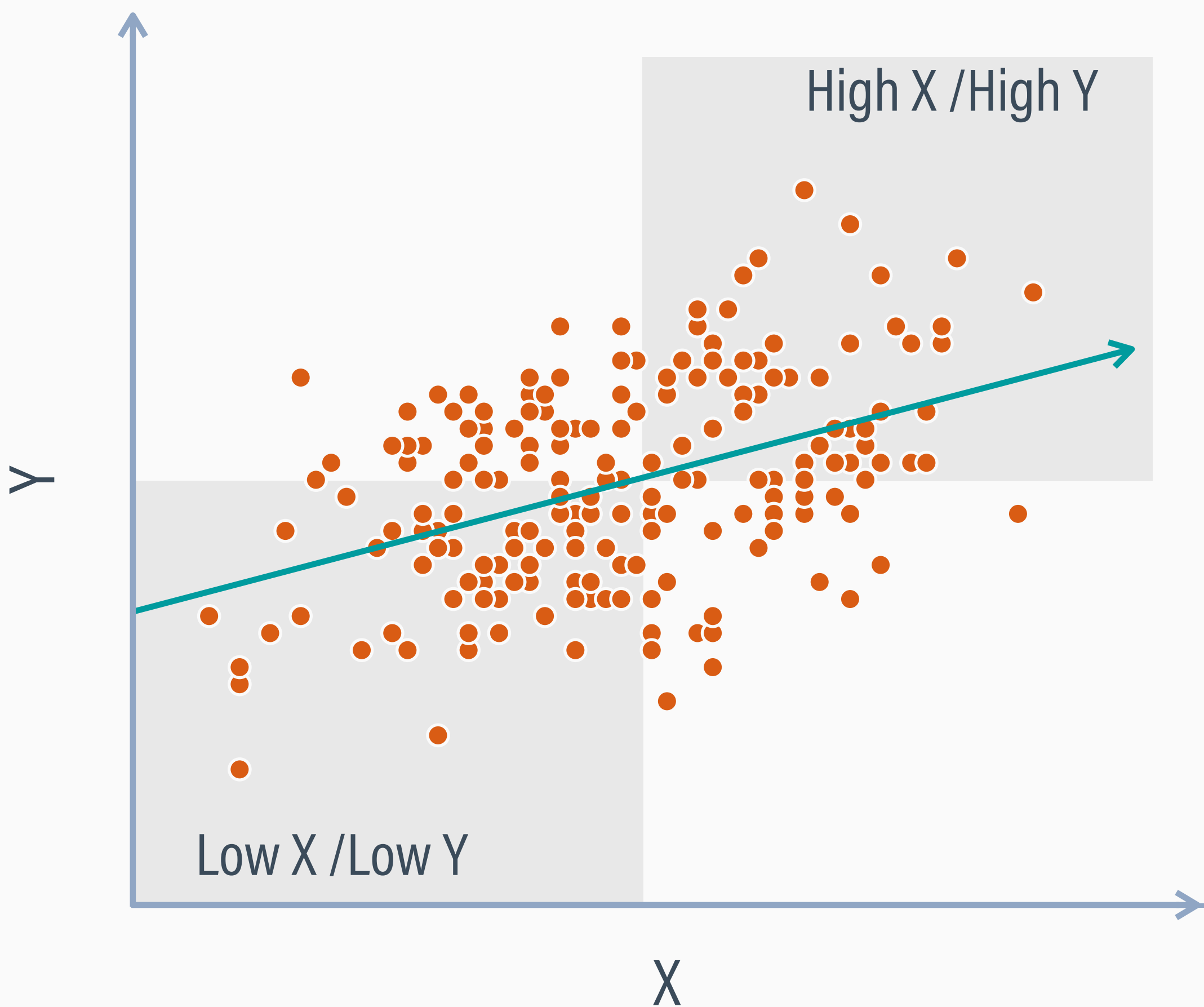
Strong positive ( r = .50 )
